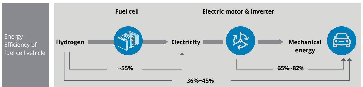
Figure 77 Energy efficiency of tank to wheels stage of FCEV
